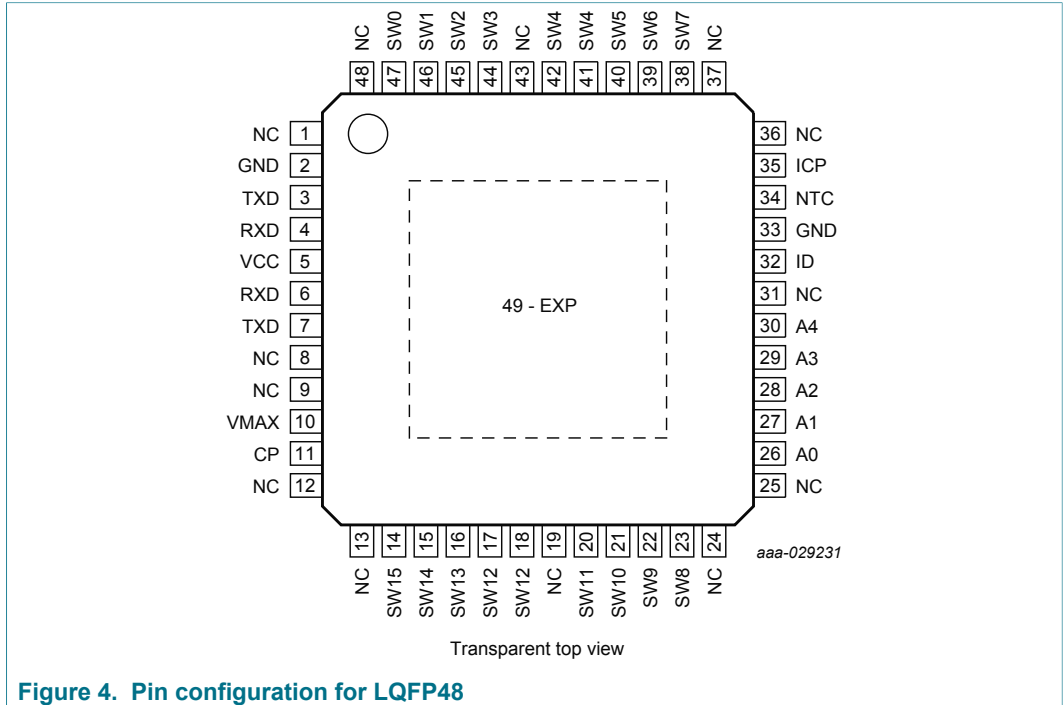
Figure 4. Pin configuration for LQFP48
