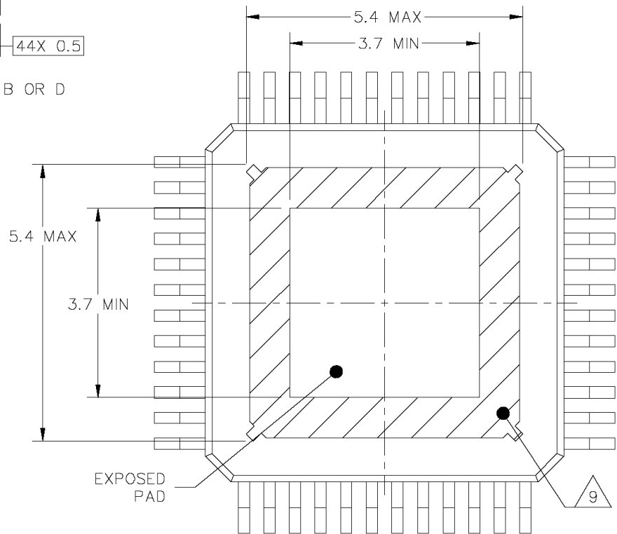
VIEW G-G
