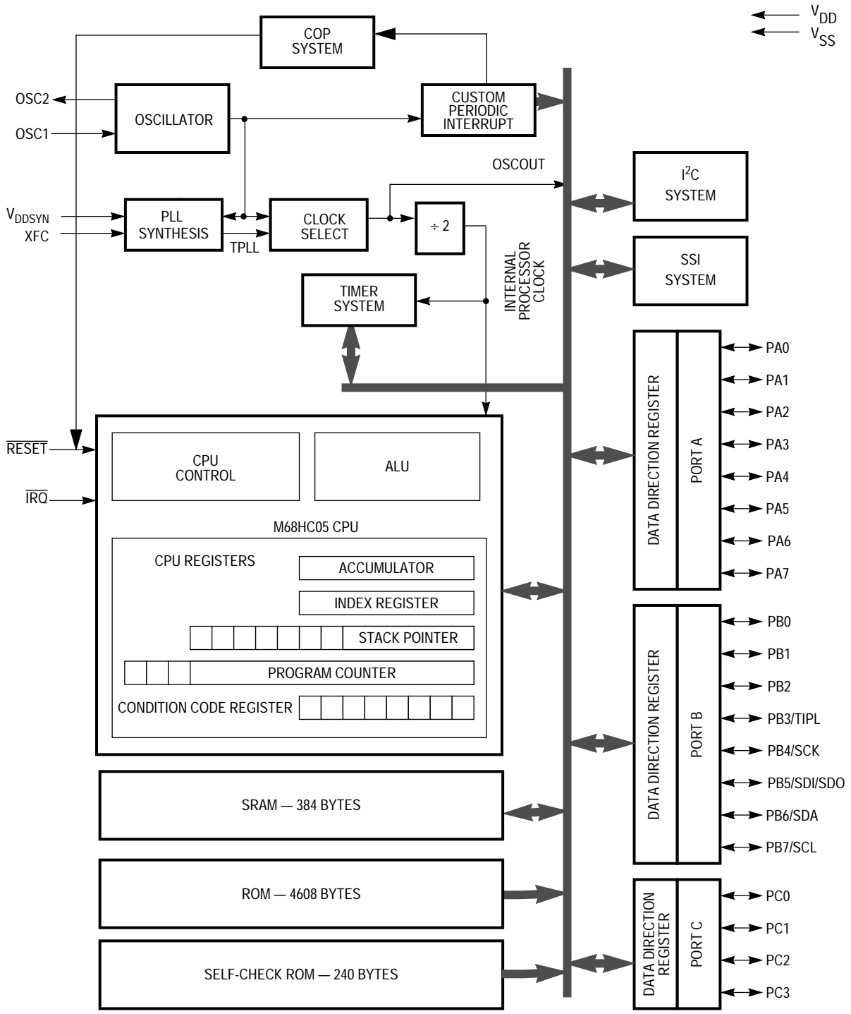
Figure 1-1. Block Diagram
