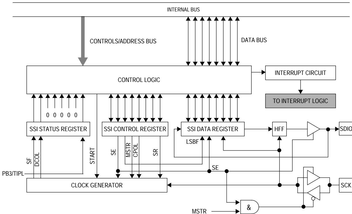
Figure 12-1. SSI Block Diagram
