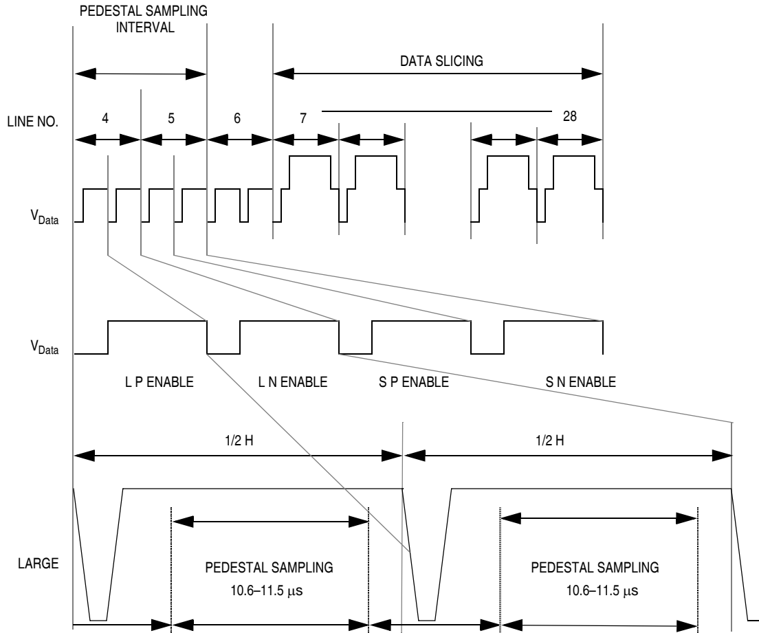
Figure 4-18. Pedestal Clamp Timing
