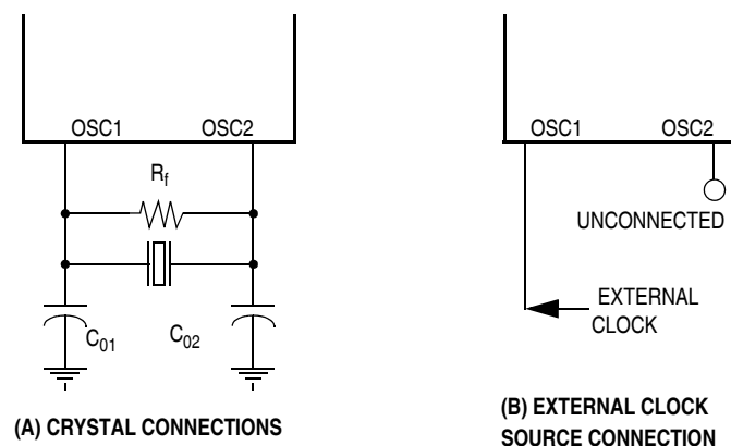
Figure 1-4. Oscillator Connections
