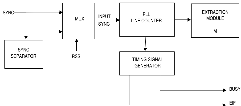
Figure 3-3. PLL Clock Signal Distribution
