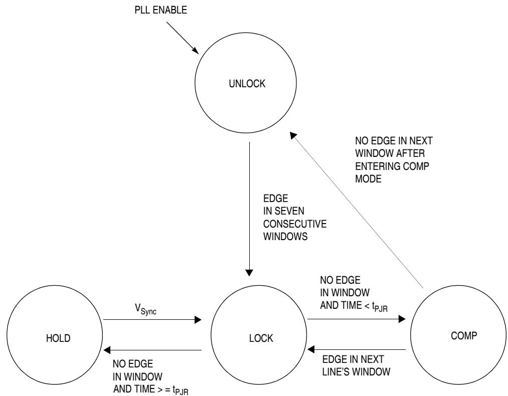
Figure 3-8. PLL State Diagram
