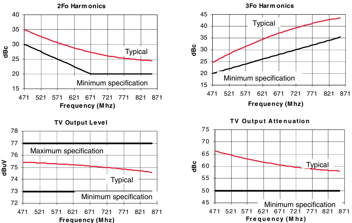
Figure 3. Typical Performance
