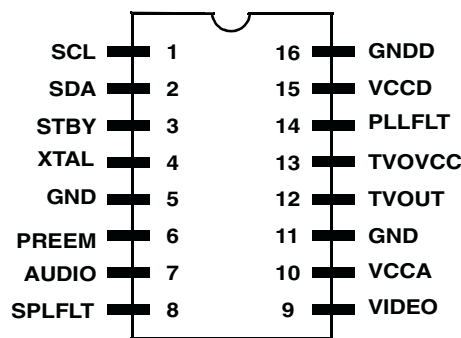
Figure 1. Pin Connections
