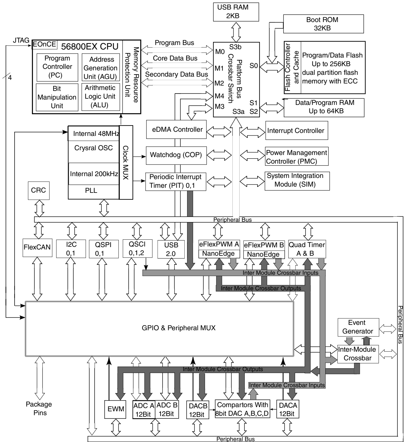
Figure 2. System diagram
