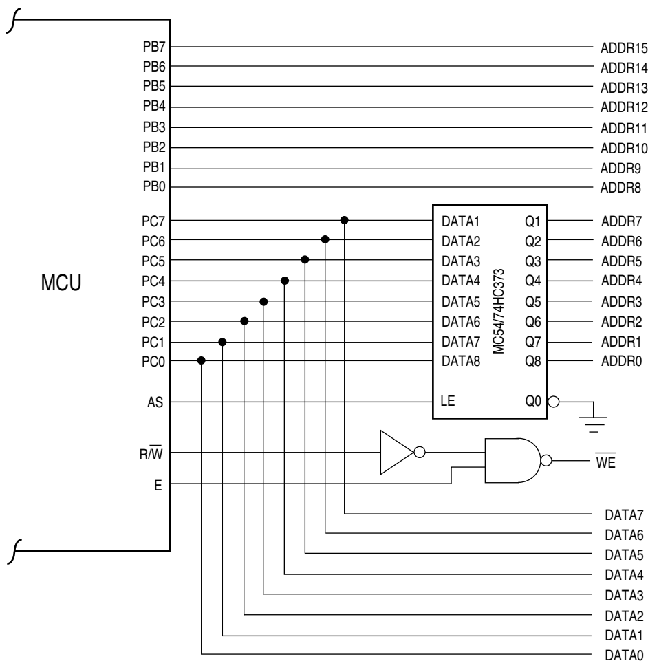
Figure 5 Address/Data Demultiplexing
