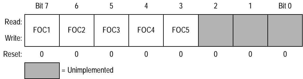
Figure 9-2. Timer Compare Force Register (CFORC)
