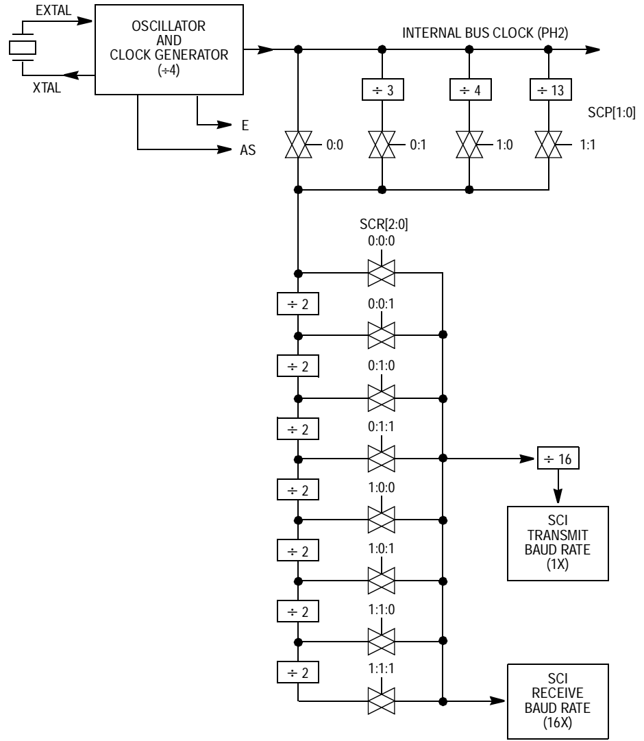
Figure 7-4. SCI Baud Rate Generator Clock Diagram
