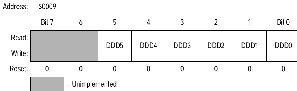
Figure 6-4. Port D Data Direction Register (DDRD)
