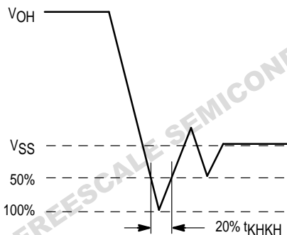
Figure 2. Undershoot Voltage
