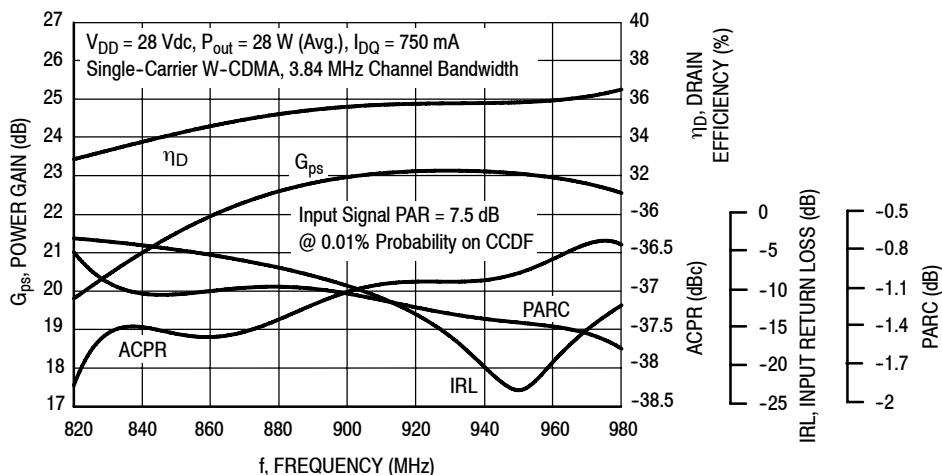
Figure 2. Output Peak-to-Average Ratio Compression (PARC) Broadband Performance @ P_{out} = 28 \text{ Watts Avg.}
