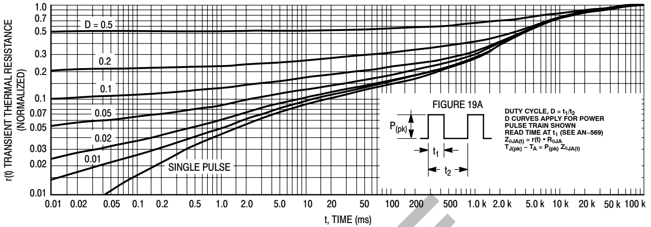
Figure 19. Thermal Response
