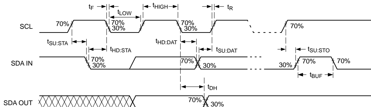
Figure 5. Bus Timing
