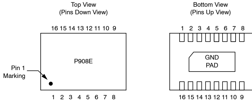
CM1692-08DE 16-Lead UDFN Package
