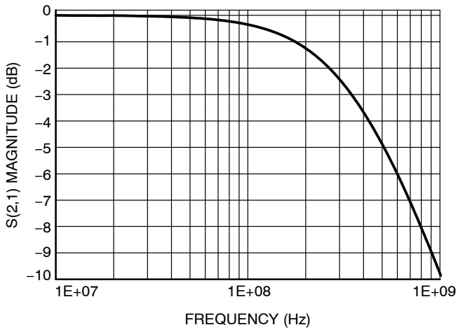
Figure 9. Insertion Loss
