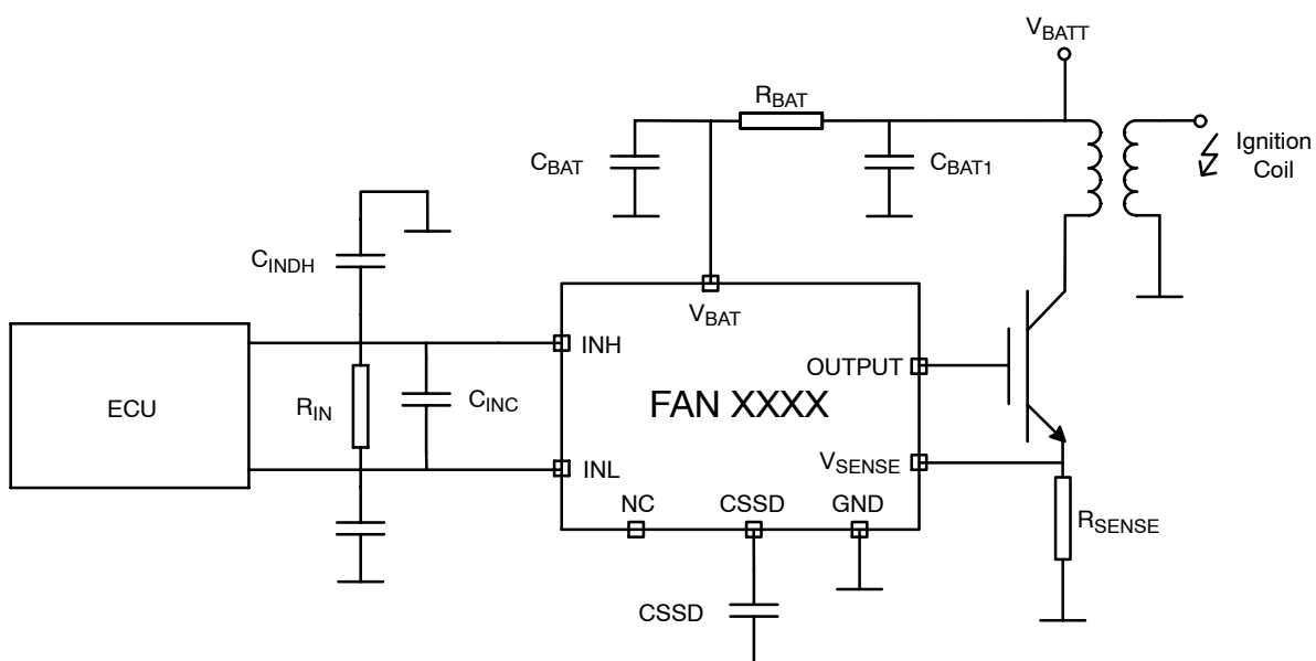
Figure 1. Typical Application
