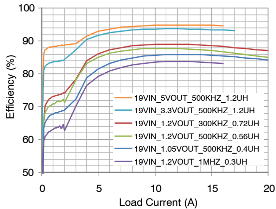
Figure 10. Efficiency vs. Load Current with V_{IN} = 19\text{ V}
