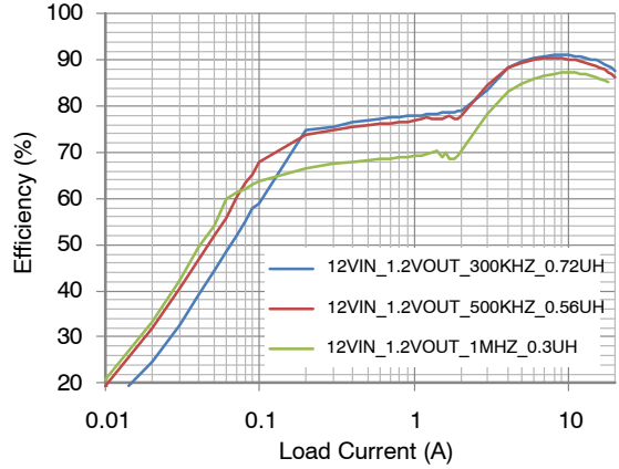
Figure 9. Efficiency vs. Load Current with V_{IN} = 12\text{ V} and V_{OUT} = 1.2\text{ V}
