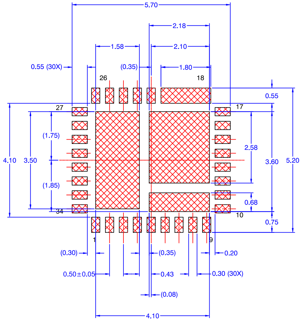
LAND PATTERN RECOMMENDATION
