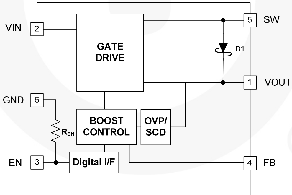
Figure 2. Block Diagram
