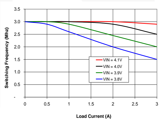
Figure 12. Effect of t_{OFF} Minimum on Reducing the Switching Frequency at Large Duty Cycles, V_{OUT} = 3.3\text{ V}
