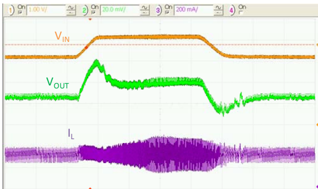
Figure 19. Line Transient at V_{IN}=3.2V to 4.2V, 300mA Load, t_{RISE}=t_{FALL}=10\mu s , 20 \mu s/div.
