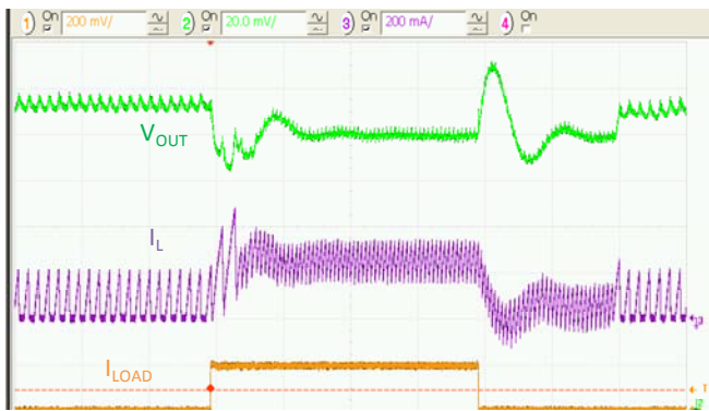
Figure 21. Load Transient 50mA to 250mA, V_{IN}=3.6V , t_{RISE}=t_{FALL}=100ns , 5 \mu s/div.
