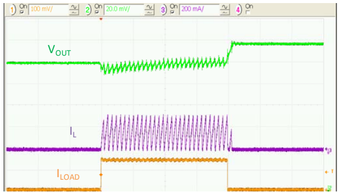
Figure 20. Load Transient 0mA to 150mA, V_{IN}=3.6V , t_{RISE}=t_{FALL}=100ns , 5 \mu s/div.
