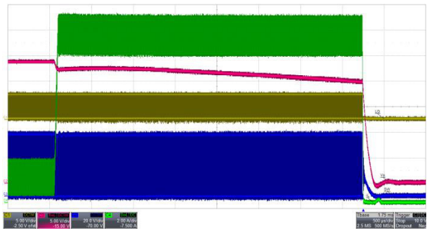
Figure 27. Over-current Protection with 280 kHz Switching Frequency
