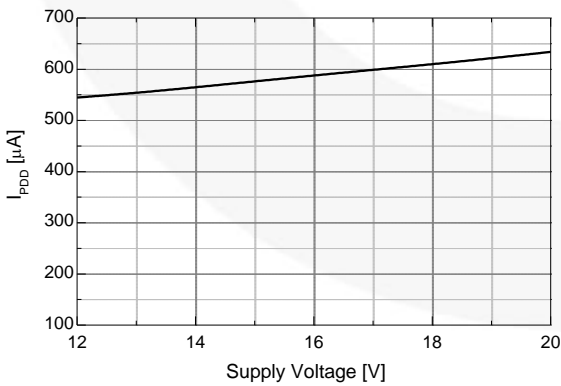
Figure 32. Operating V DD Supply Current vs. Supply Voltage
