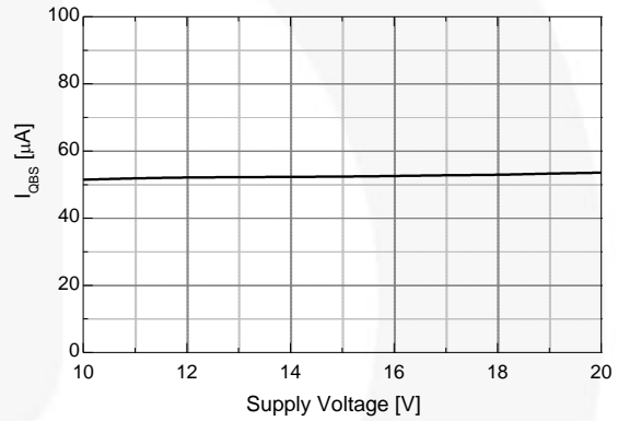
Figure 31. Quiescent V BS Supply Current vs. Supply Voltage
