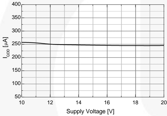
Figure 30. Quiescent V DD Supply Current vs. Supply Voltage
