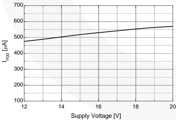
Figure 33. Operating V_{DD} Supply Current vs. Supply Voltage
