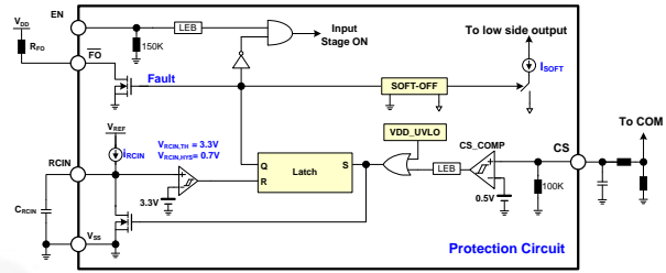
Figure 43. Over-Current Protection
