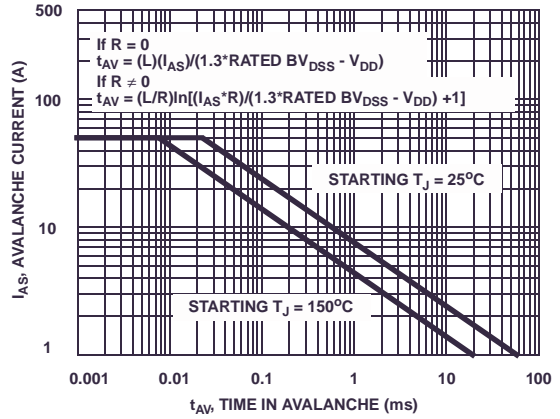
Figure 6. Unclamped Inductive Switching Capability NOTE: Refer to N and d Application Notes AN7514 and AN7515
