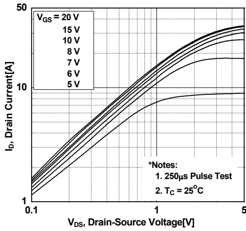
Figure 1. On-Region Characteristics
