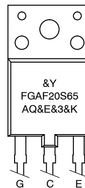
TO-3PF CASE 340AH
