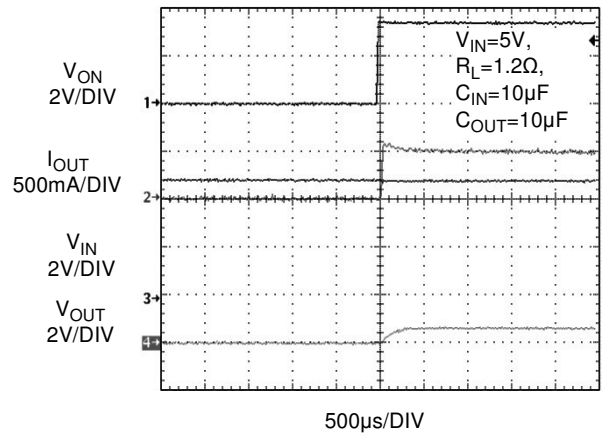
Figure 18. Current Limit Response (Output is loaded with 1.2Ω resistor and C OUT =10μF)
