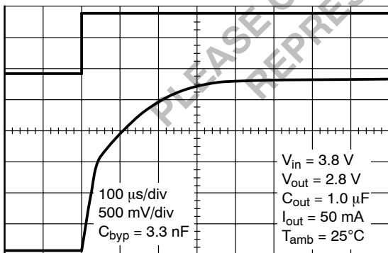
Figure 20. Output Voltage Settling Shape Cbypass = 3.3 nF
