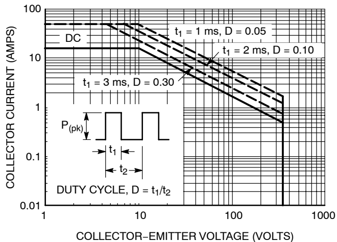
Figure 19. Pulse Train Safe Operating Area (Mounted on an Infinite Heatsink at T_C = 25^\circ\text{C} )
