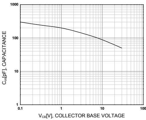
Figure 3. Collector Capacitance
