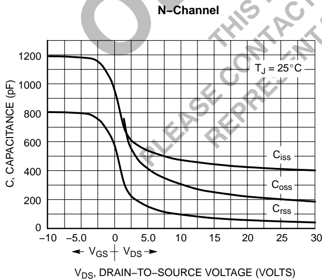
Figure 7. Capacitance Variation
