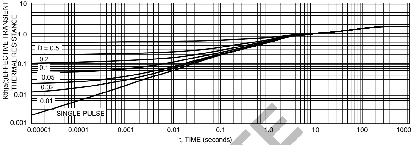
Figure 14. Thermal Response
