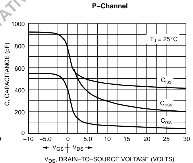
Figure 7. Capacitance Variation
