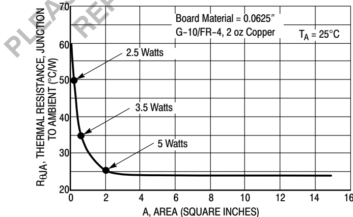
Figure 17. Thermal Resistance versus Drain Pad Area for the D 2 PAK Package (Typical)
