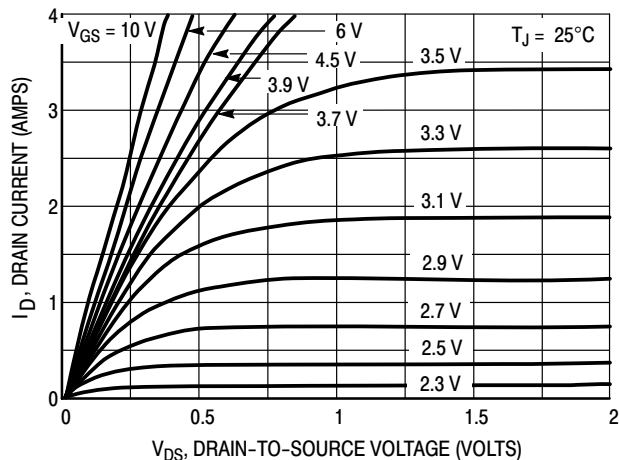
Figure 3. On-Region Characteristics
