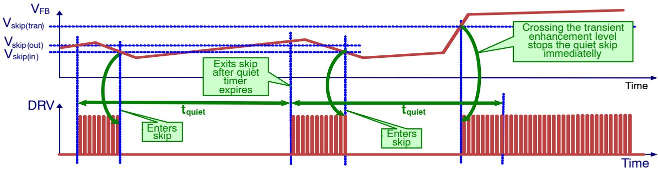
Figure 62. Leaving the Quiet-Skip Mode during Load Transient
