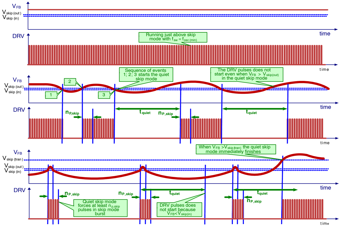
Figure 63. Quiet-Skip Timing Diagram - Option
