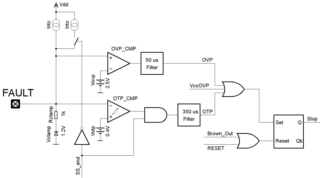
Figure 73. OVP/OTP Detection Schematic
