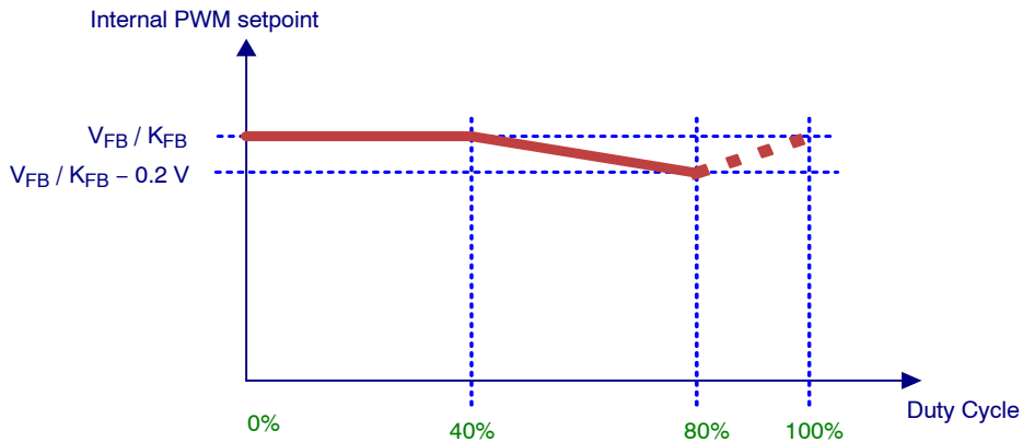
Figure 66. Slope Compensation Timing Diagram
