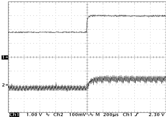
Upper Trace: Battery Voltage, V_{IN} , 1.0 V/Division Lower Trace: Output Voltage Ripple, 100 mV/Division
