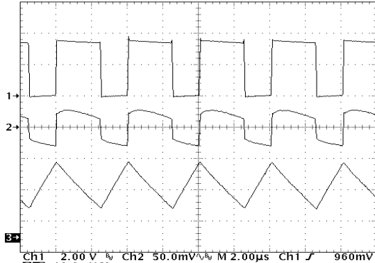
Upper Trace: Voltage at L_X pin, 2.0 V/Division Middle Trace: Output Voltage Ripple, 50 mV/Division Lower Trace: Inductor Current, I_L , 100 mA/Division
