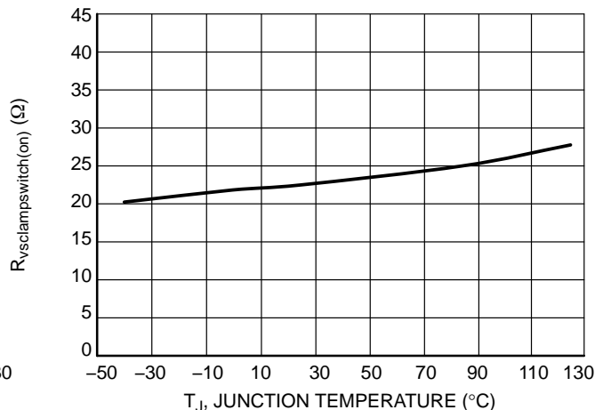
Figure 35. Volt-Second Switch-On Resistance Variation vs. Junction Temperature
