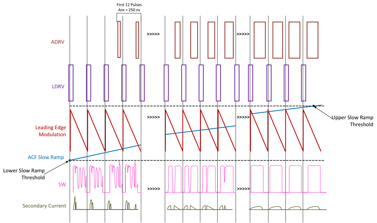
Figure 16. Leading Edge Modulation of ADRV During DCM to ACF Transition
