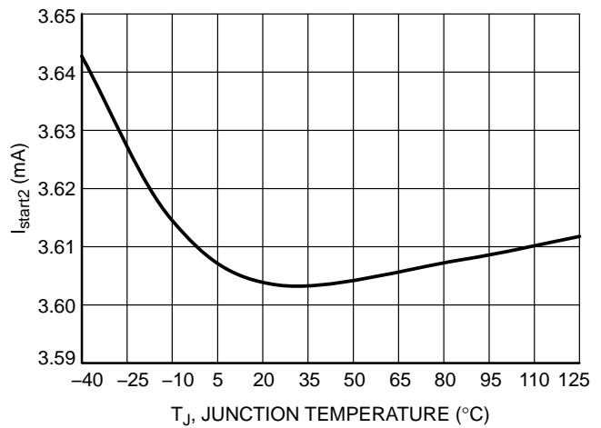
Figure 36. I start2 vs. Temperature
