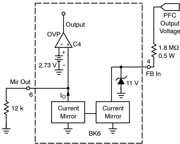
Figure 43. Overvoltage Protection
