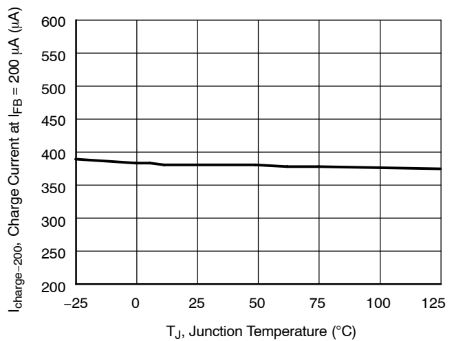
Figure 20. Charge Current at I FB = 200 µA vs. Junction Temperature
