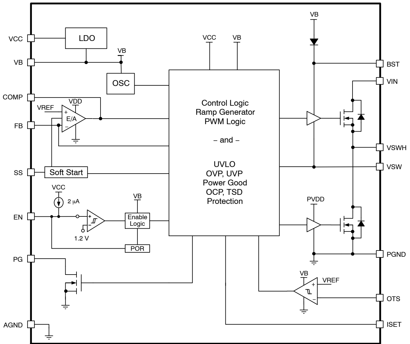
Figure 1. NCP3231N Block Diagram
