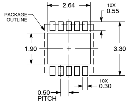
DIMENSIONS: MILLIMETERS
