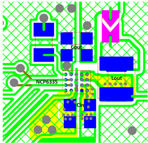
Figure 62. Demo Board Example
