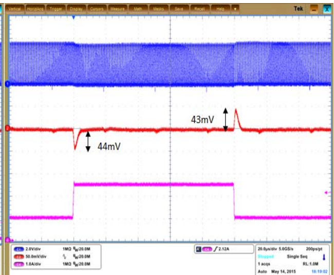
Figure 43. Transient Load 1.0 – 2.5 A Auto Mode
