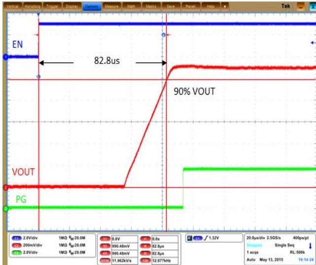
Figure 40. Normal Power Up, V_{OUT}=1.1\text{ V} , No Load
