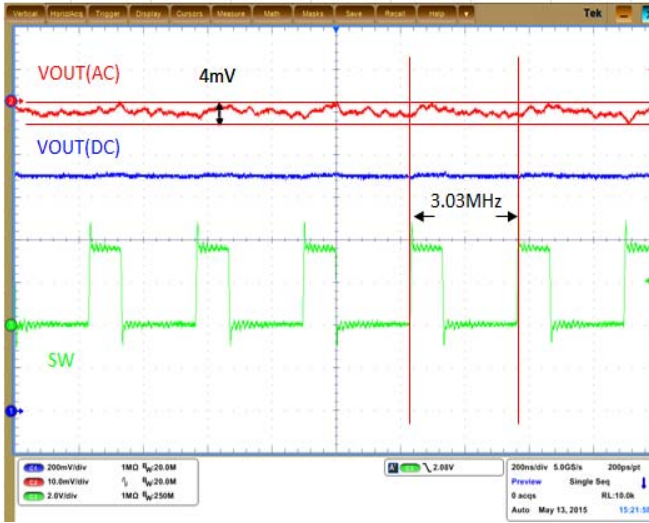
Figure 38. PWM Ripple, V_{OUT}=1.1\text{ V} , No load
