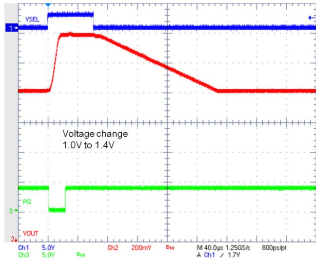
Figure 25. DVS Transition 1.0V – 1.39375 V
