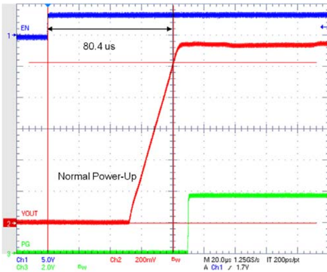
Figure 24. Normal Power Up, V_{OUT} = 1.15\text{ V}
