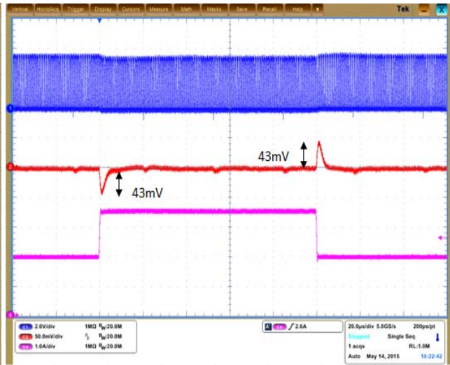
Figure 45. Transient Load 2.0 – 3.5 A Auto Mode
