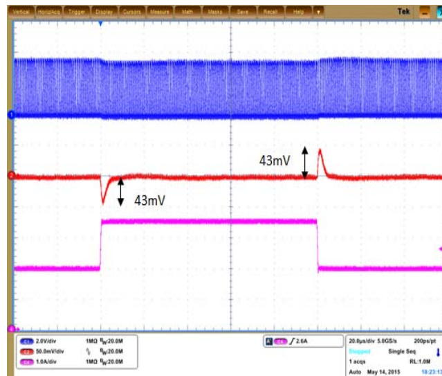
Figure 46. Transient Load 2.0 – 3.5 A Forced PWM Mode
