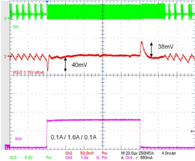
Figure 26. Transient Load 0.1 – 1.6 A Auto Mode
