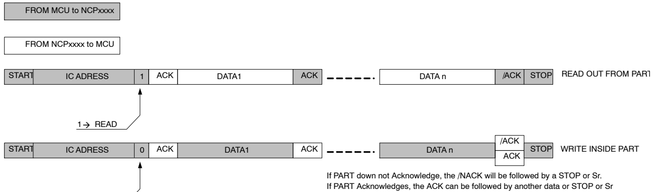
Figure 56. General Protocol Description
