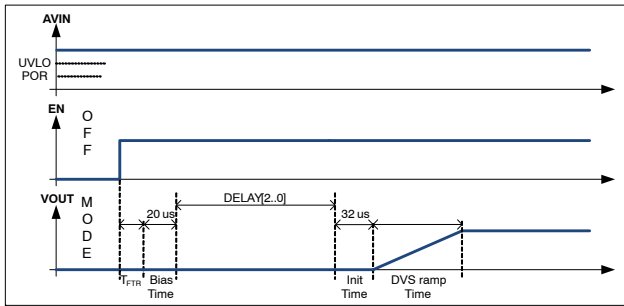
Figure 48. Normal Power Up Sequence
