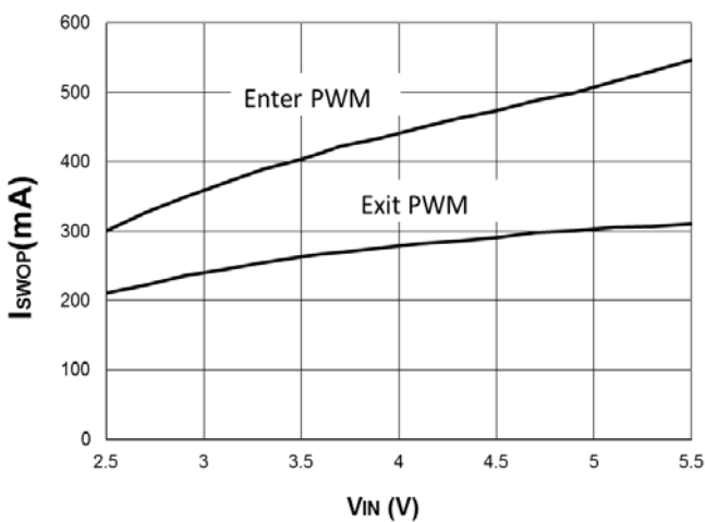
Figure 36. Switchover Point V_{OUT} = 1.1\text{ V}
