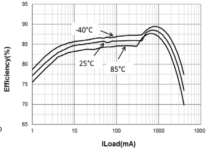
Figure 33. Efficiency vs I_{LOAD} and Temperature V_{OUT} = 1.1\text{ V} , PIFE20161B Inductor
