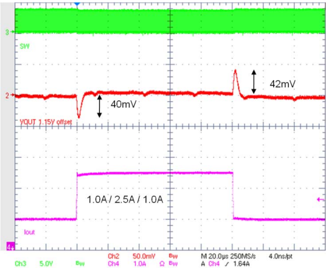
Figure 28. Transient Load 1.0 – 2.5 A Auto Mode
