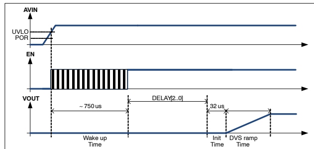
Figure 47. Initial Power Up Sequence
