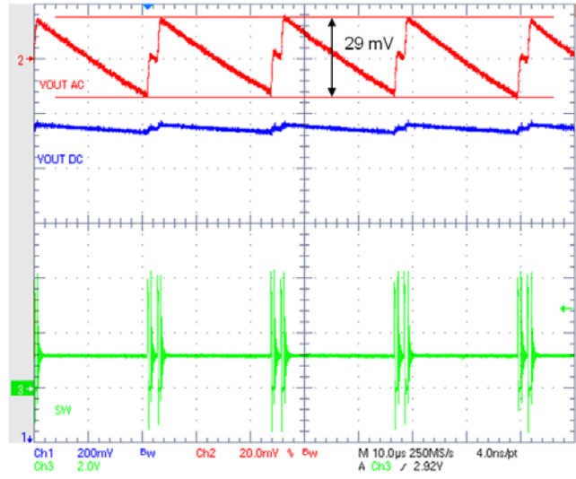
Figure 23. PFM Ripple
