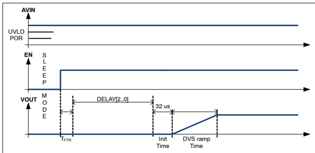
Figure 49. Quick Power Up Sequence
