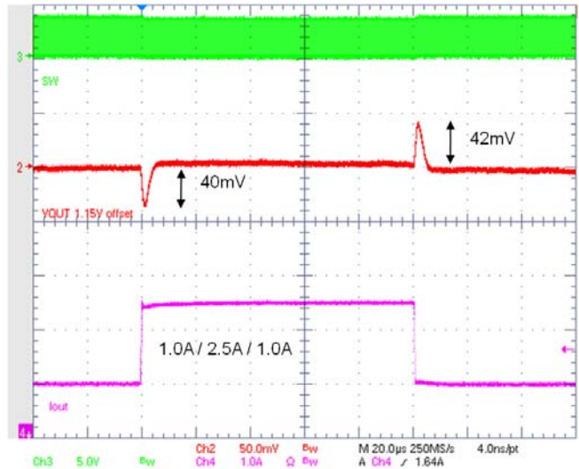
Figure 29. Transient Load 1.0 – 2.5 A Forced PWM Mode
