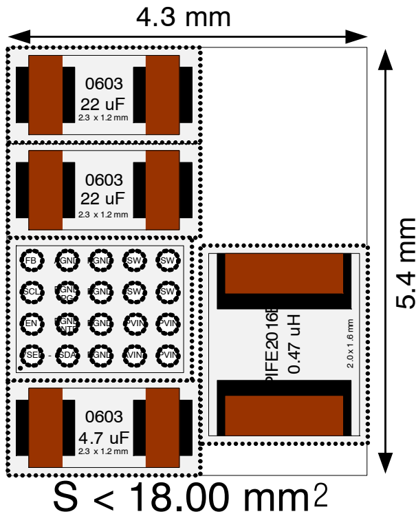
Figure 61. Layout Recommendation
