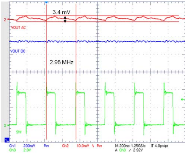
Figure 22. PWM Ripple
