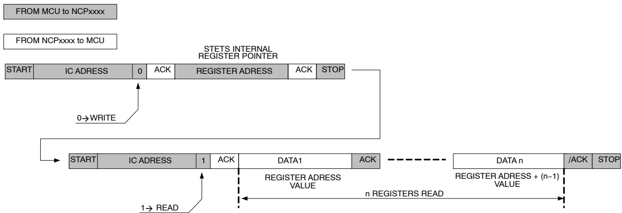
Figure 57. Read Out from Part
