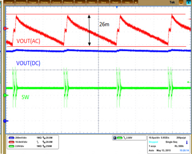
Figure 39. PFM Ripple, V_{OUT}=1.1\text{ V} , I_{Load}=20\text{ mA}
