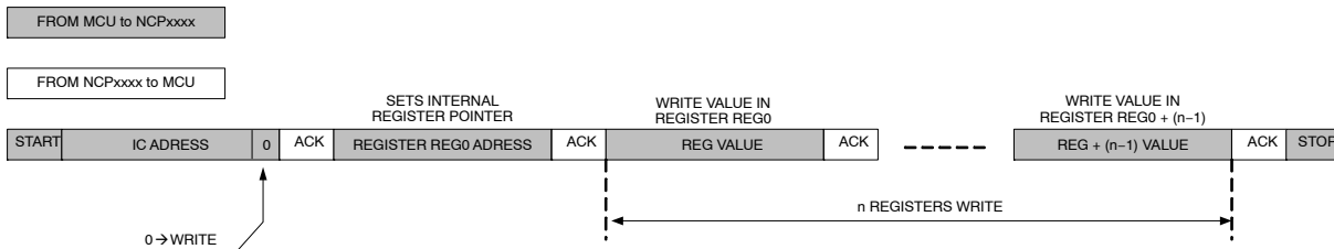
Figure 59. Write in n Registers
