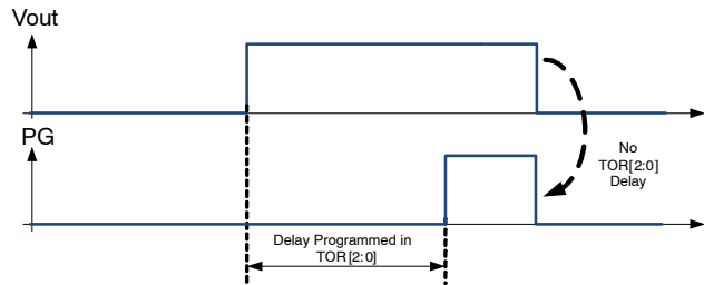
Figure 54. Power Good Operation
