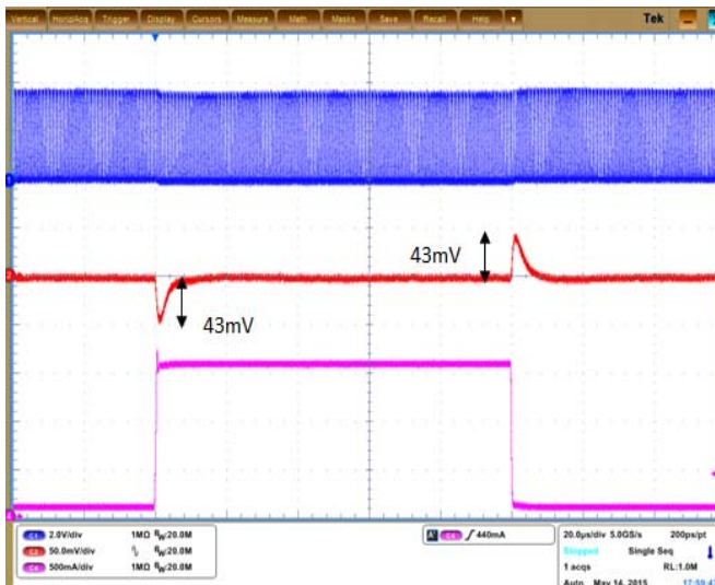
Figure 42. Transient Load 0.1 – 1.6 A Forced PWM Mode
