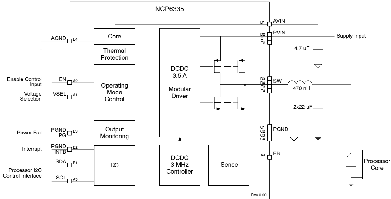
Figure 60. Typical Application Schematic
