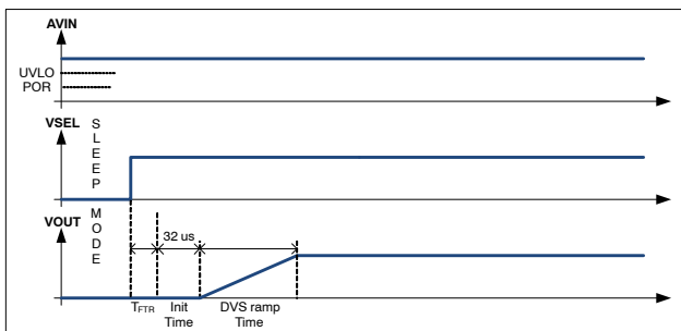
Figure 50. Fast Power Up Sequence
