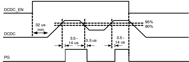
Figure 53. Power Good signal
