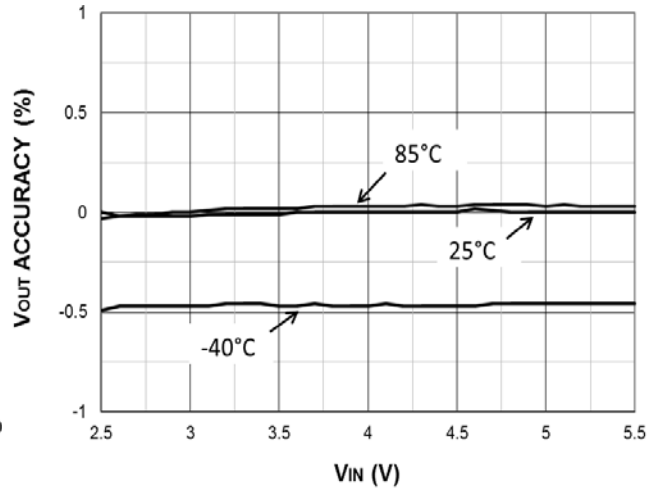
Figure 35. V_{OUT} Accuracy vs V_{IN} and Temperature V_{OUT} = 1.1\text{ V} , I_{LOAD} = 2.0\text{ A}
