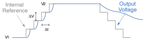
Figure 52. DVS in Auto Mode Diagram
