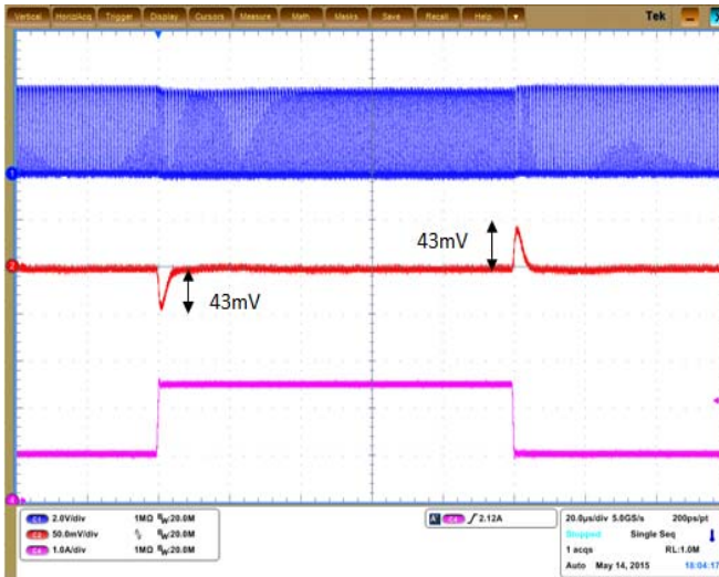
Figure 44. Transient Load 1.0 – 2.5 A Forced PWM Mode
