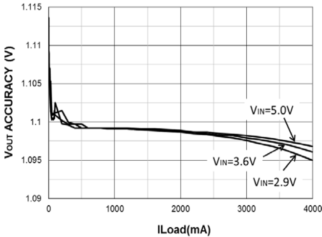
Figure 34. V_{OUT} Accuracy vs I_{LOAD} and V_{IN} V_{OUT} = 1.1\text{ V}
