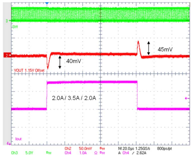
Figure 31. Transient Load 2.0 – 3.5 A Forced PWM Mode
