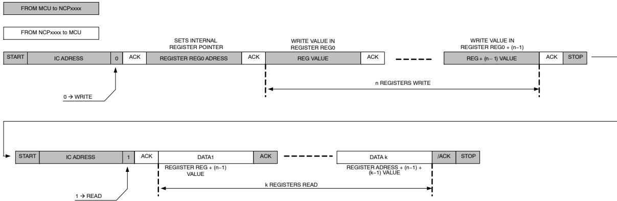
Figure 58. Write Followed by Read Transaction
