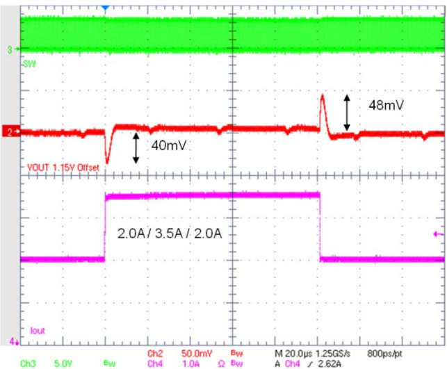
Figure 30. Transient Load 2.0 – 3.5 A Auto Mode
