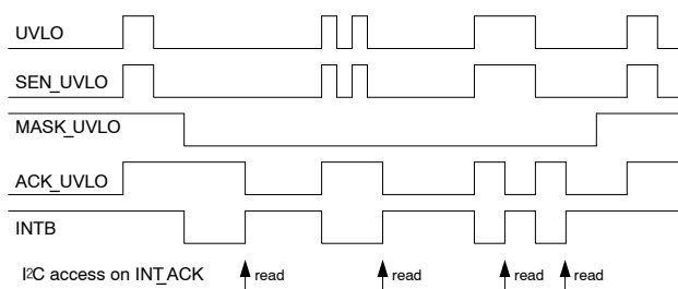
Figure 55. Interrupt Operation Example
