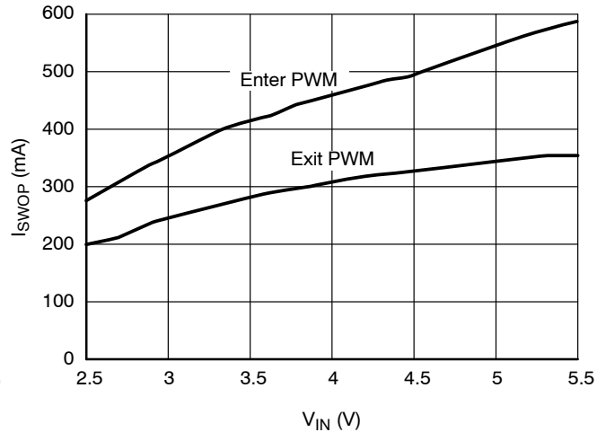
Figure 37. Switchover Point V_{OUT} = 1.39375\text{ V}
