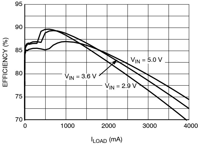
Figure 32. Efficiency vs I_{LOAD} and V_{IN} V_{OUT} = 1.1\text{ V} , PIFE20161B Inductor
