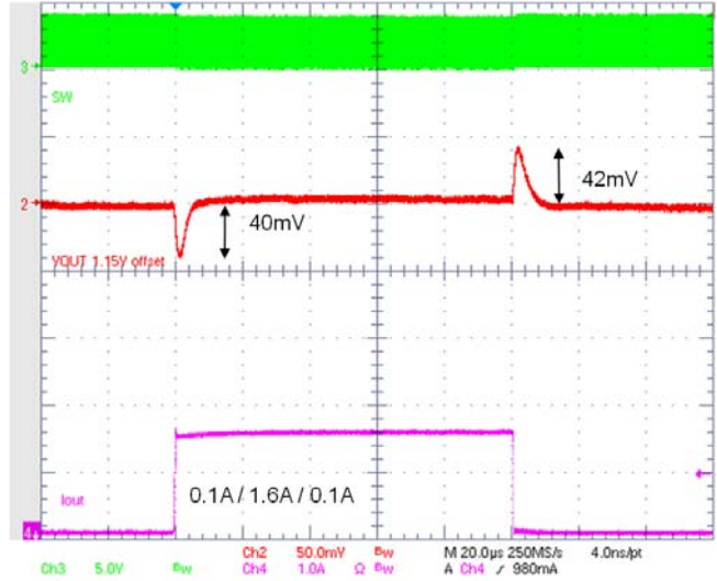
Figure 27. Transient Load 0.1 – 1.6 A Forced PWM Mode
