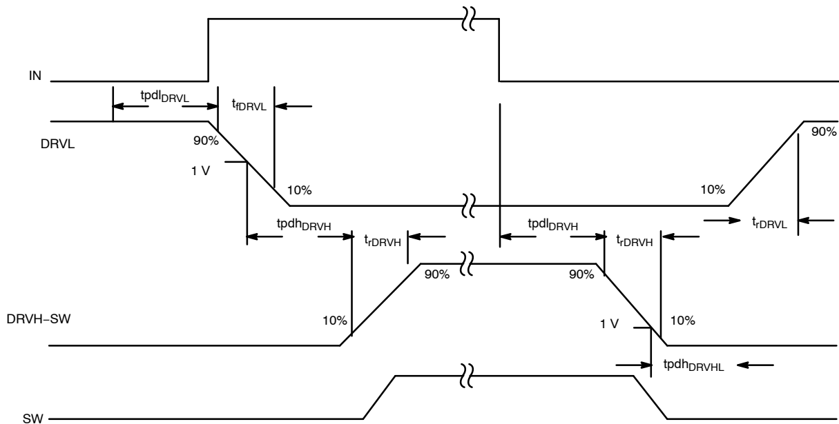
Figure 3. Timing Diagram
