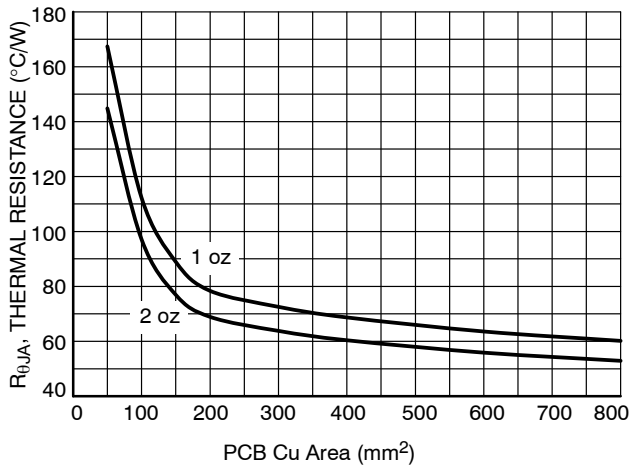
Figure 26. R_{\theta JA} vs. PCB Cu Area (DPAK Package)
