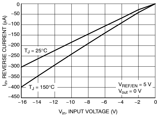
Figure 14. Reverse Current vs. Input Voltage
