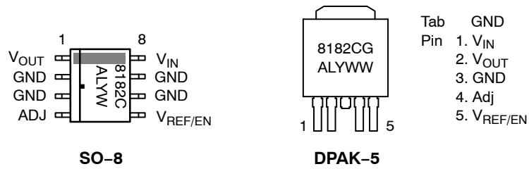
Figure 3. Pin Connections
