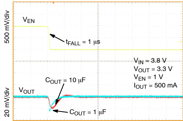
10 μs/div Figure 51. Line Transient Response – Falling Edge, V_{OUT} = 3.3 V , I_{OUT} = 500 mA
