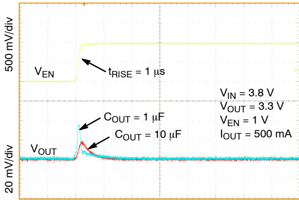
5 μs/div Figure 50. Line Transient Response – Rising Edge, V_{OUT} = 3.3 V , I_{OUT} = 500 mA
