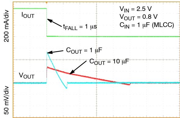
100 μs/div Figure 53. Load Transient Response – Falling Edge, V_{OUT} = 0.8 V , I_{OUT} = 1 mA to 500 mA , C_{OUT} = 1 μF , 10 μF
