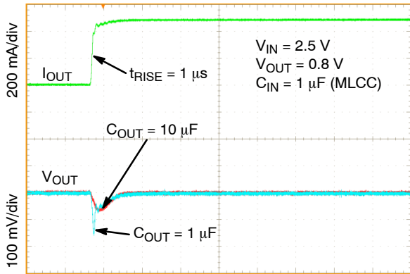
10 μs/div Figure 52. Load Transient Response – Rising Edge, V_{OUT} = 0.8 V , I_{OUT} = 1 mA to 500 mA , C_{OUT} = 1 μF , 10 μF
