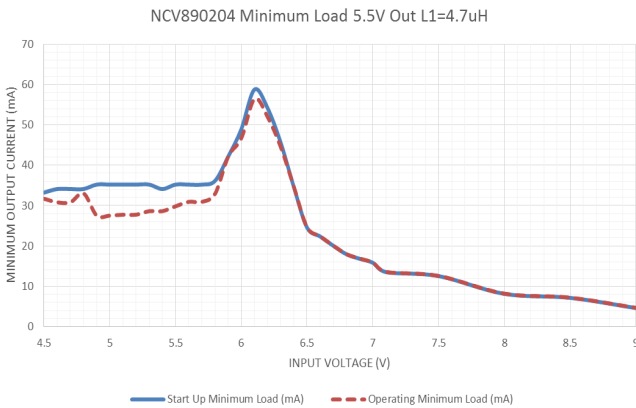
Typical Minimum Load 5.5 V Out, L1 = 4.7 µH
