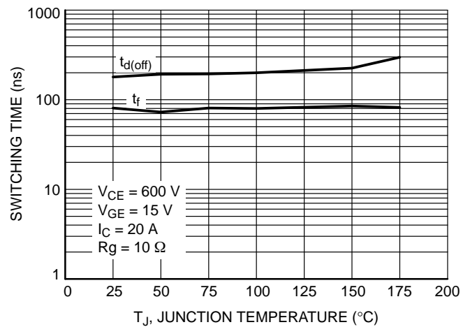
Figure 12. Switching Time vs. Temperature
