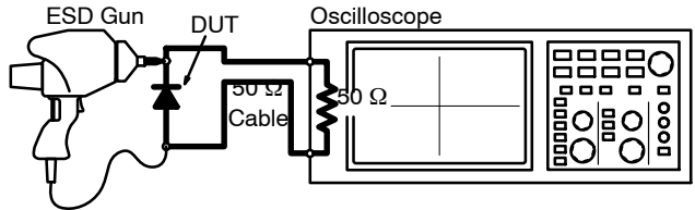
Figure 13. Diagram of ESD Test Setup
