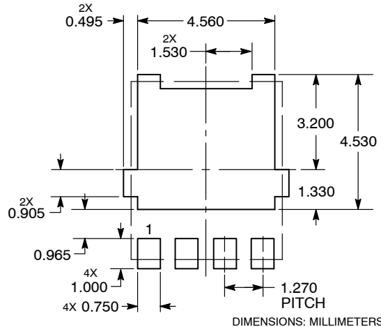
DIMENSIONS: MILLIMETERS
