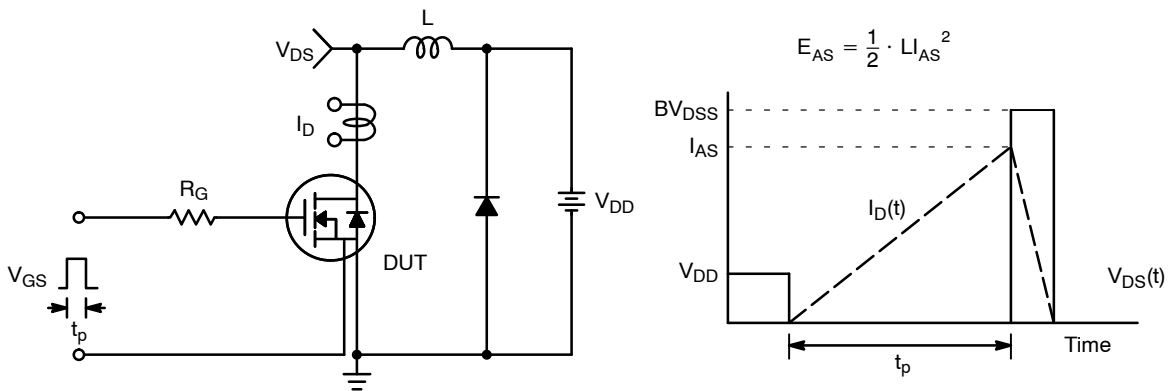
Figure 14. Unclamped Inductive Switching Test Circuit & Waveforms
