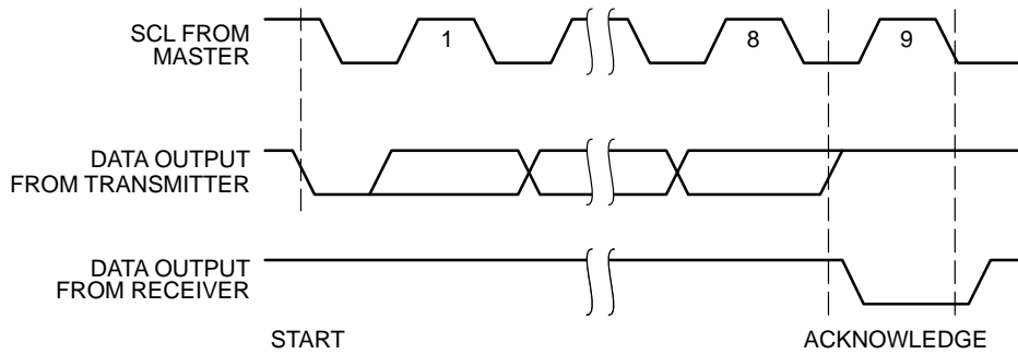
Figure 3. Acknowledge Timing
