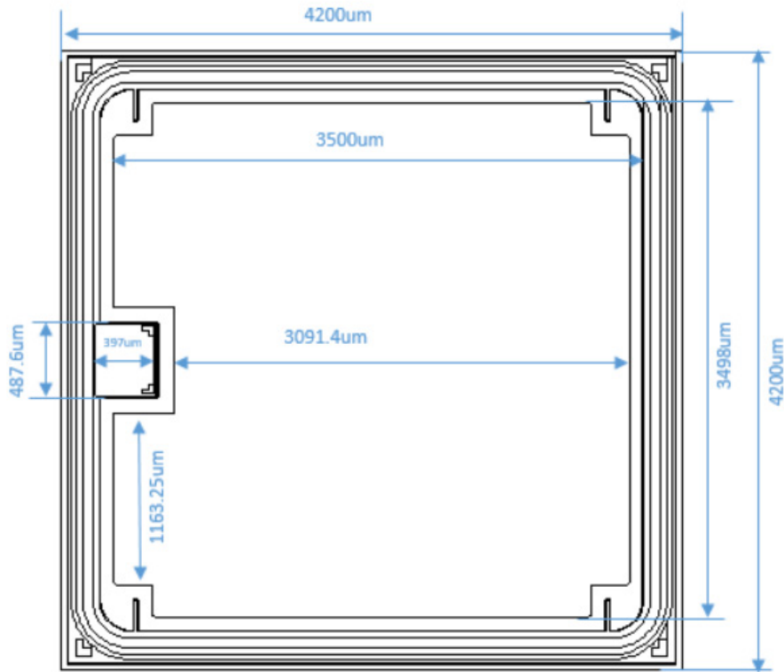
Figure 1. Die Layout
