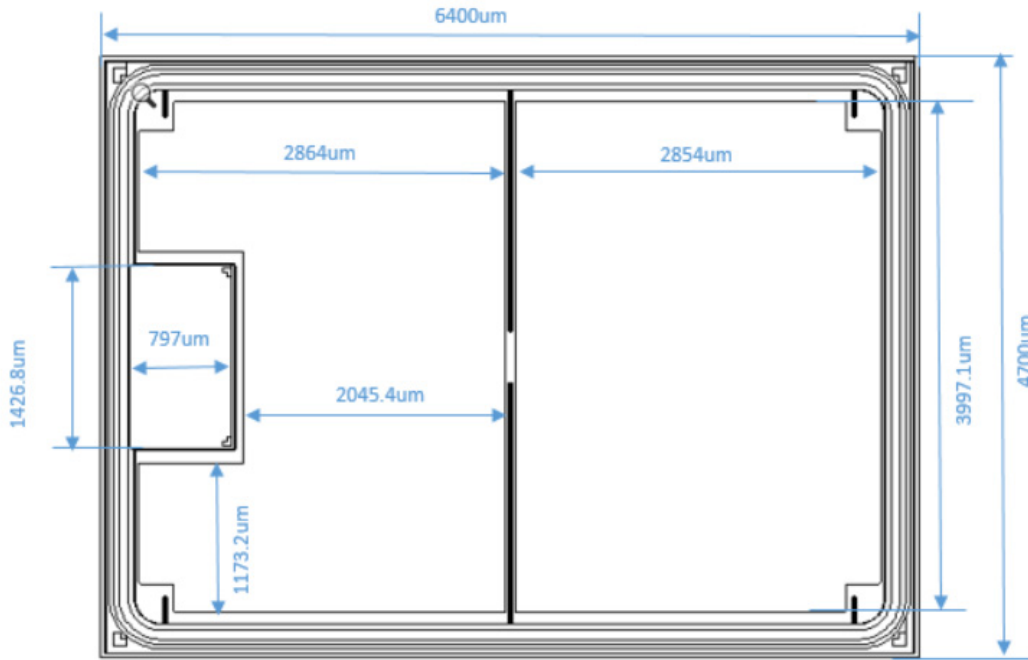
Figure 1. Die Layout
